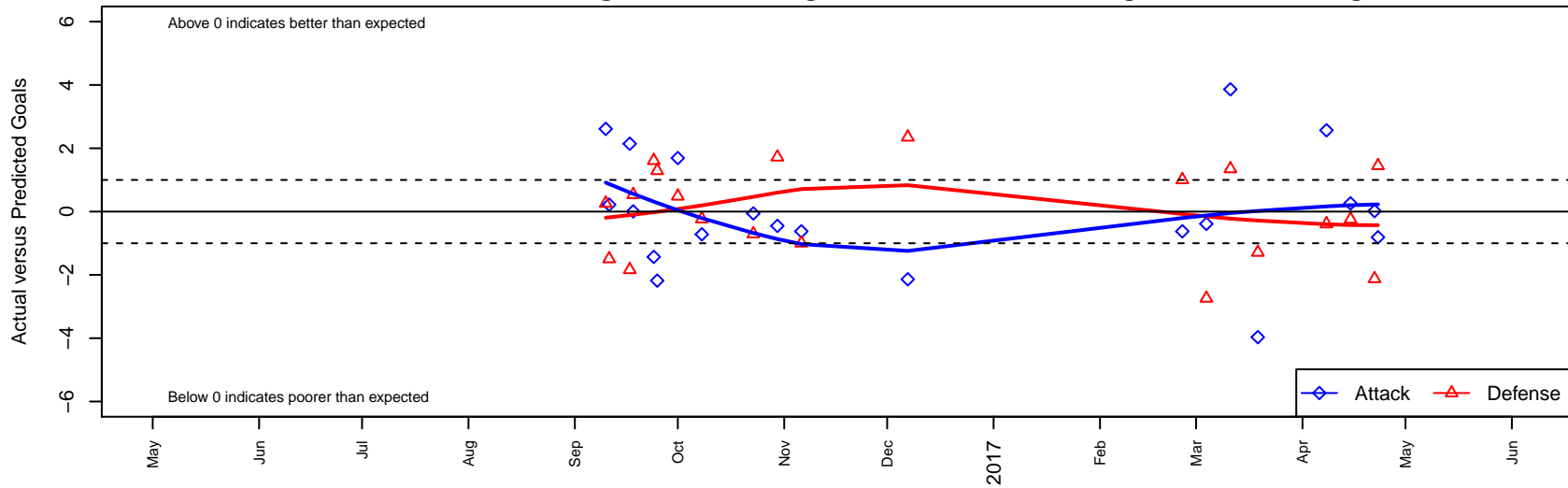
BSC Portland Black B04 Dots are actual minus expected GF (blue circles) and GA (red triangles). Blue line is smoothed change in attack strength. Red is smoothed change in defense strength.
